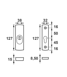
Solo Solid Flex Premium Rozeta
