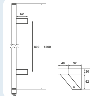
Amsterdam Skos 120 cm
