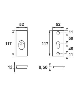
Solo Royal++ Flex Rozeta
