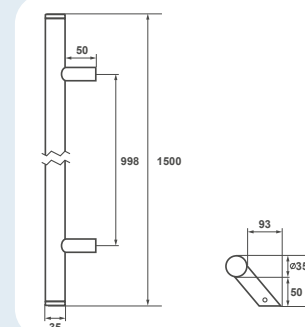
Amsterdam Prosta 150 cm
