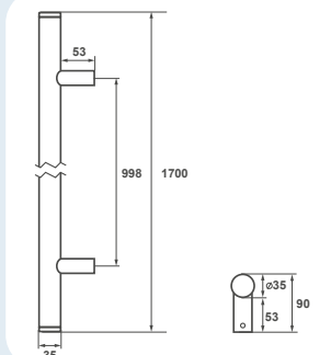
Montreal Prosta 170 cm
