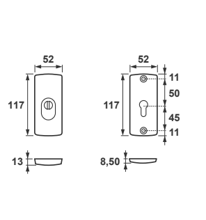
Solo Jupiter Electro Flex Premium Rozeta
