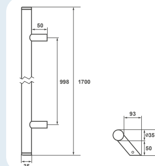
Montreal Skos 170 cm
