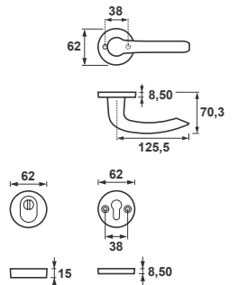
Solo Solid Flex Premium Rozeta
