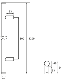
Montreal Prosta 120 cm
