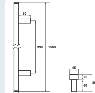
Amsterdam Prosta 150 cm
