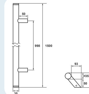
Amsterdam Prosta 150 cm
