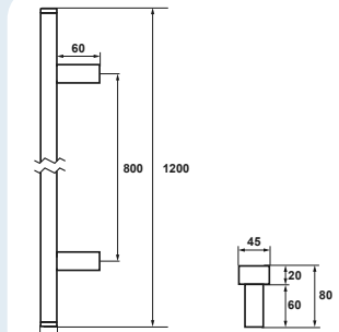
Amsterdam Prosta 120 cm
